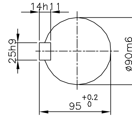
OUTPUT SHAFT
