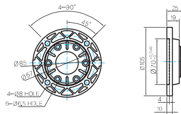
● MODEL: 040-Flange-71B14
