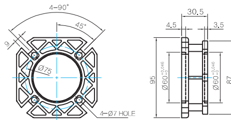
● MODEL: WHG-040-Fa
