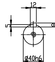
OUTPUT SHAFT
