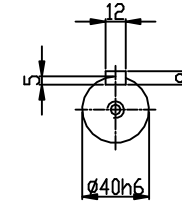
OUTPUT SHAFT
