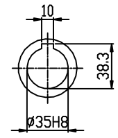
OUTPUT SHAFT
