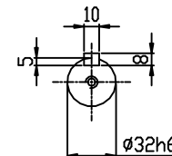
OUTPUT SHAFT
