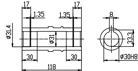
OUTPUT SHAFT
