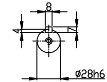
OUTPUT SHAFT
