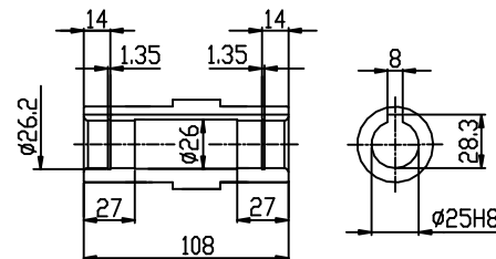
OUTPUT SHAFT
