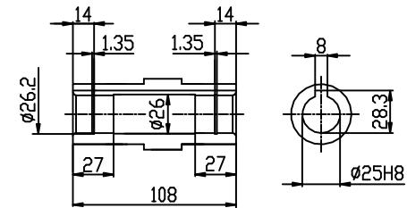
OUTPUT SHAFT
