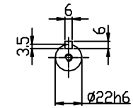
OUTPUT SHAFT
