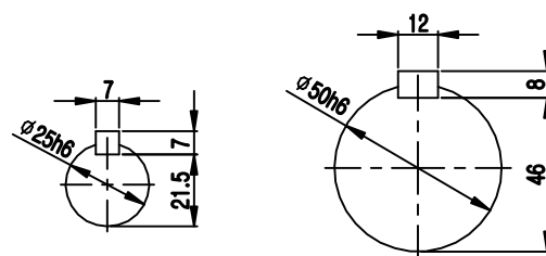
OUTPUT SHAFT
