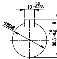
OUTPUT SHAFT
