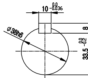
OUTPUT SHAFT
