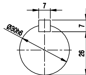
OUTPUT SHAFT
