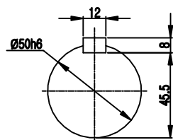
OUTPUT SHAFT
