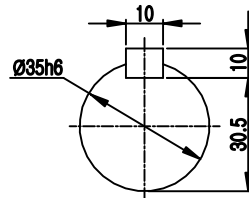
OUTPUT SHAFT
