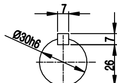
OUTPUT SHAFT
