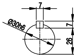
OUTPUT SHAFT
