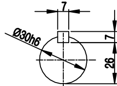
OUTPUT SHAFT
