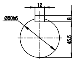
OUTPUT SHAFT
