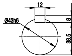
OUTPUT SHAFT
