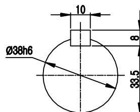
OUTPUT SHAFT
