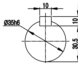
OUTPUT SHAFT
