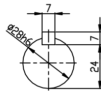
OUTPUT SHAFT
