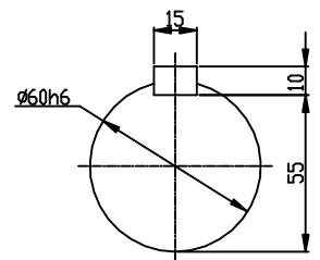
OUTPUT SHAFT
