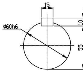
OUTPUT SHAFT
