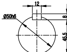
OUTPUT SHAFT
