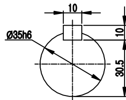
OUTPUT SHAFT
