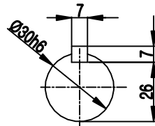
OUTPUT SHAFT
