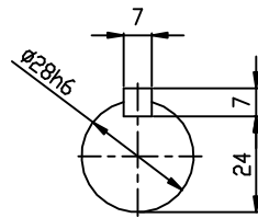
OUTPUT SHAFT
