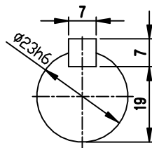
OUTPUT SHAFT
