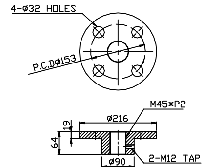
FLANGE NUT (SCALE:1/2)
