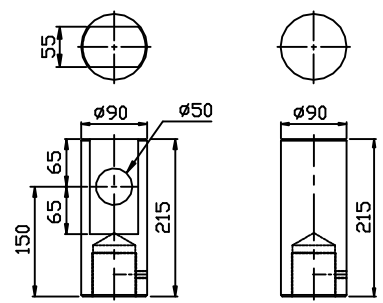
CLEVIS NUT (SCALE:1/2) PLAIN NUT (SCALE:1/2)
