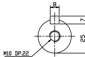
OUTPUT SHAFT
