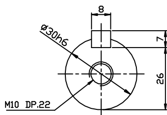
OUTPUT SHAFT
