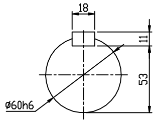
OUTPUT SHAFT
