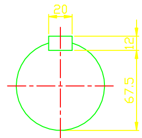
OUTPUT SHAFT
