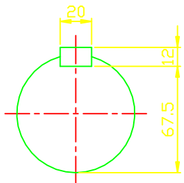
OUTPUT SHAFT
