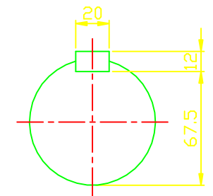
OUTPUT SHAFT
