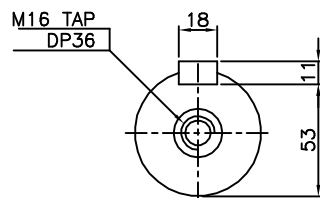
OUTPUT SHAFT
