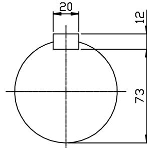
OUTPUT SHAFT
