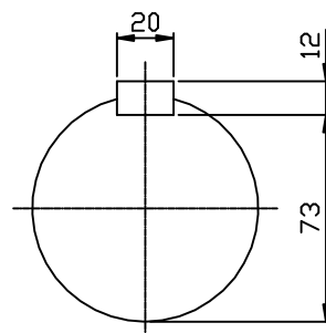
OUTPUT SHAFT
