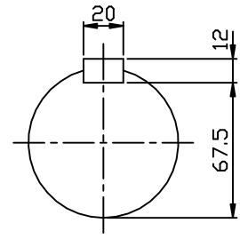
OUTPUT SHAFT
