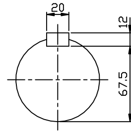
OUTPUT SHAFT
