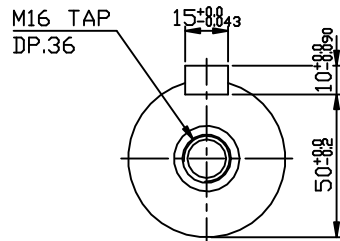
OUTPUT SHAFT
