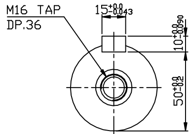
OUTPUT SHAFT
