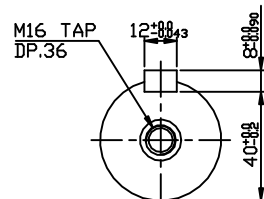
OUTPUT SHAFT
