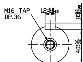
OUTPUT SHAFT
