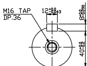
OUTPUT SHAFT
