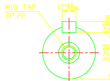
OUTPUT SHAFT
